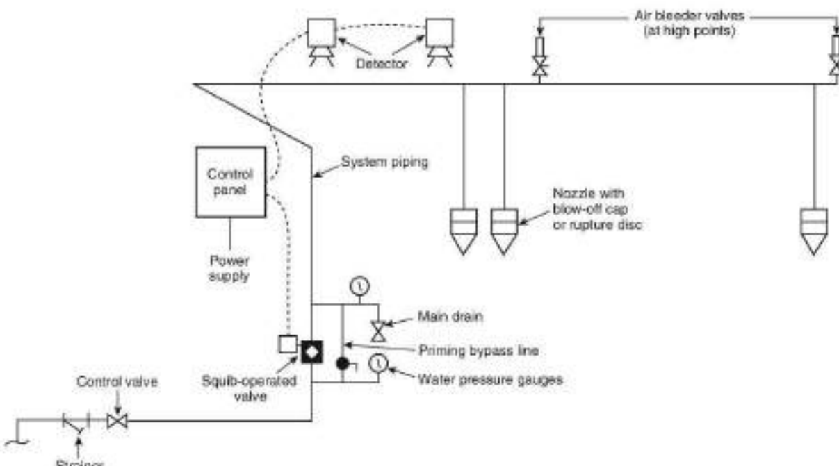
FIGURE A.12.3.10(a) Ultra-High-Speed System Using Squib-Operated Valve.
