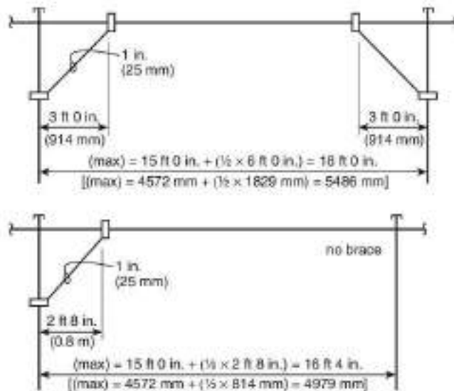
FIGURE A.6.3.2.2.5 Sway/Support Brace.
