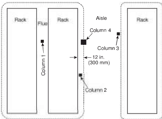
▲ FIGURE A.20.18.1 Protection of Columns Within and Adjacent to Rack Structure.
