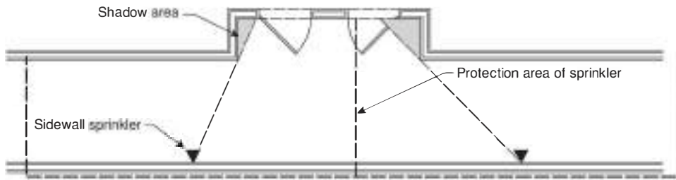
Δ FIGURE A.9.1.1(3)(a) Shadow Area in Corridor.
