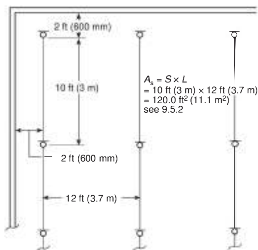
Δ FIGURE A.28.2.4.6.2 Sprinkler Spacing.
