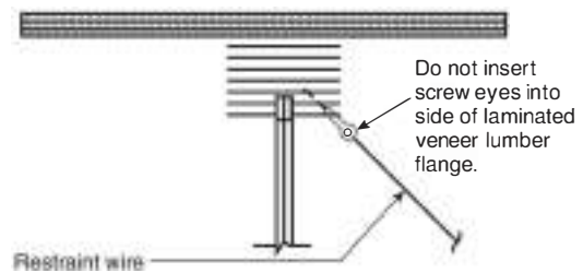
Detail F — Laminated veneer lumber upper flange
