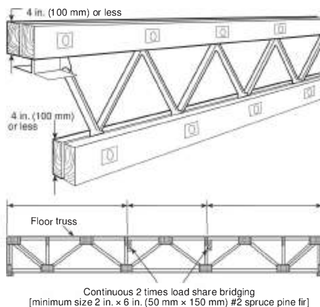
Δ FIGURE A.3.3.43.2(c) Examples of Wood Truss Construction.
