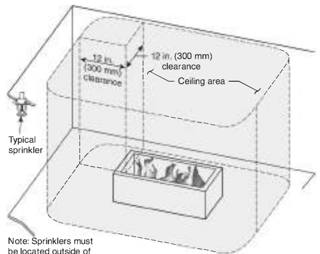
FIGURE A.9.4.2.5(d) Intermediate-Temperature Sprinkler over Open Fireplace.
