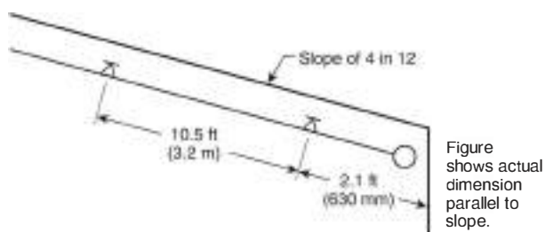
Δ FIGURE A.28.2.4.6.5 Determination of Floor Area Under Sloped Ceiling/Roof.
