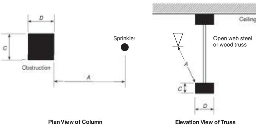
FIGURE 13.2.8.2.1.3 Minimum Distance from Obstruction (CMSA Sprinklers).
