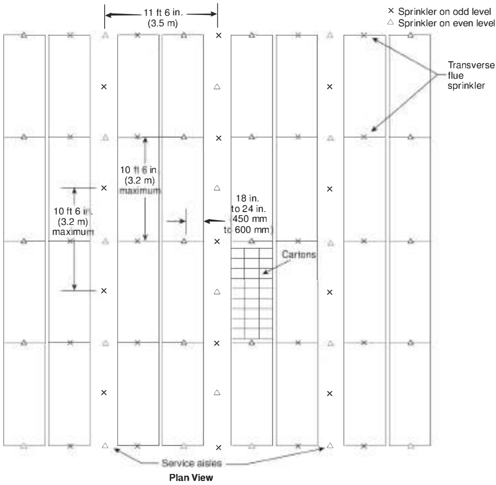
Δ FIGURE A.26.6.3.5(b) Plan View of Sprinkler Locations in Cartoned Record Storage.
