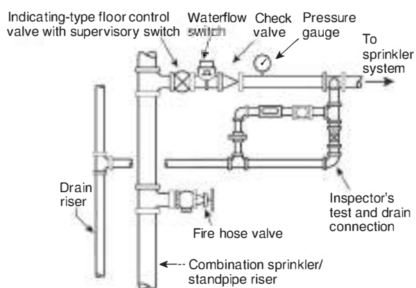
N FIGURE A.16.15.2.2(c) Acceptable Piping Arrangement for Combined Sprinkler/Standpipe System.
