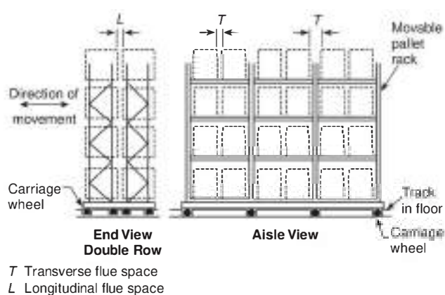
FIGURE A.3.3.177(k) Movable Rack.
