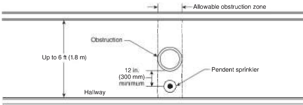
N FIGURE 11.2.5.1.2(d) Obstruction in Hallway
