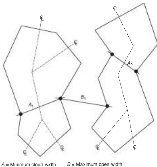
Δ FIGURE A.9.2.7.2.5 Irregular Shaped Cloud Dimensioning.
