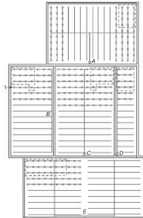
FIGURE A.28.2.4.1(a) Example of Hydraulically Most Demanding Area.
