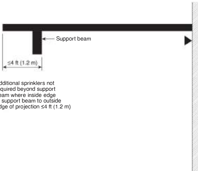
FIGURE A.9.3.19.1 Exterior Projection with Sprinklers.
