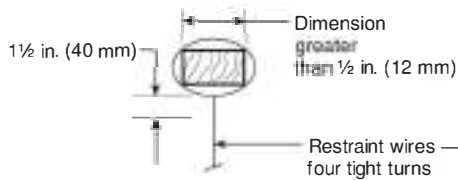
Detail G — Typical saddle tie
