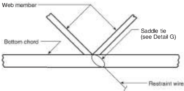
Detail E — Restraint wire parallel to wood truss
