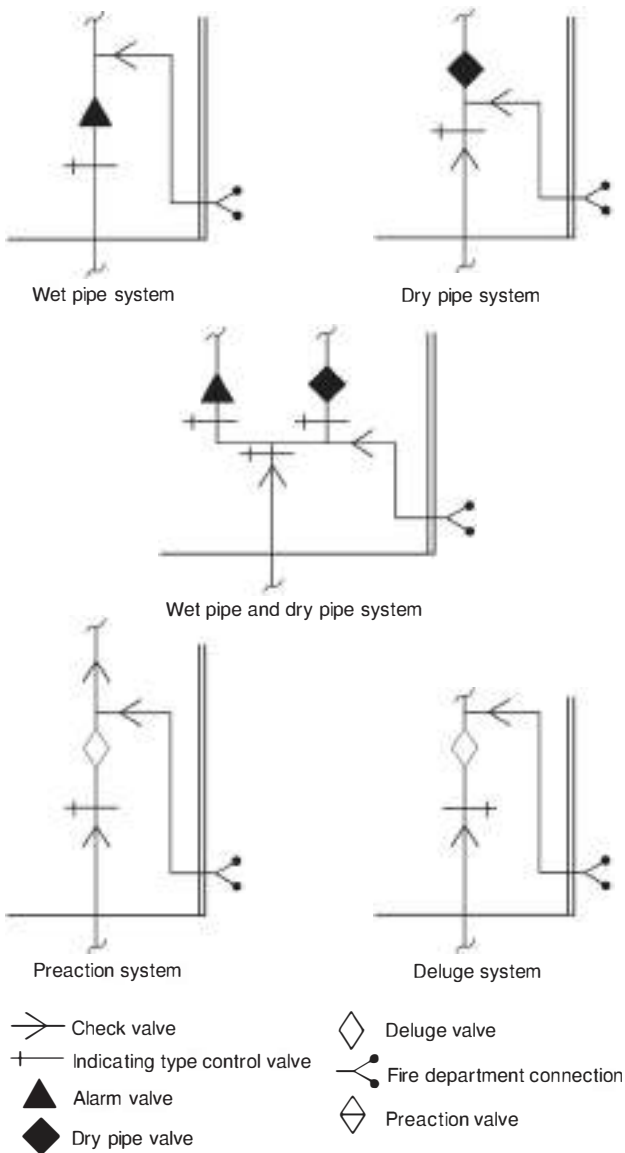
FIGURE A.16.9.3 Examples of Acceptable Valve Arrangements.
