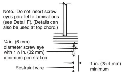
Detail H — Laminated veneer lumber lower flange
