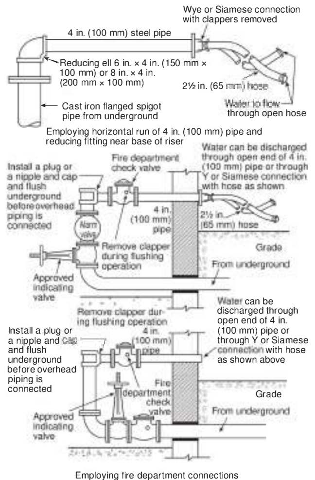
Δ FIGURE A.6.10.2.1 Methods of Flushing Water Supply Connections. [24:Figure A.10.10.2.1]
