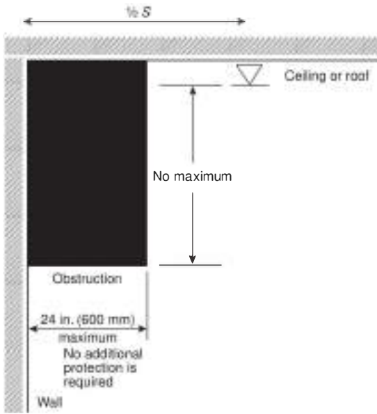
Δ FIGURE 11.2.5.1.2(c) Obstructions Against Walls (Extended Coverage Upright and Pendent Spray Sprinklers).
