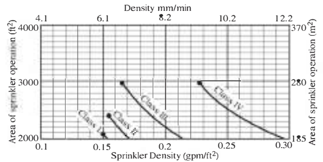
Δ FIGURE 21.2.2.3.2 For the Evaluation or Modification of Existing Systems, Sprinkler System Design Curves for 20 ft (6.1 m) High Storage — High Temperature-Rated Sprinklers.
