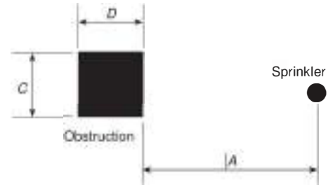
Plan View of Column (Obstruction in vertical orientation) A \geq 4C or 4D (Use dimension C or D , whichever is greater)
