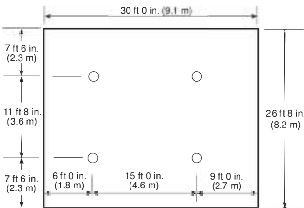
FIGURE A.10.2.5.2.3(d) Small Room Provision — Four Sprinklers.
