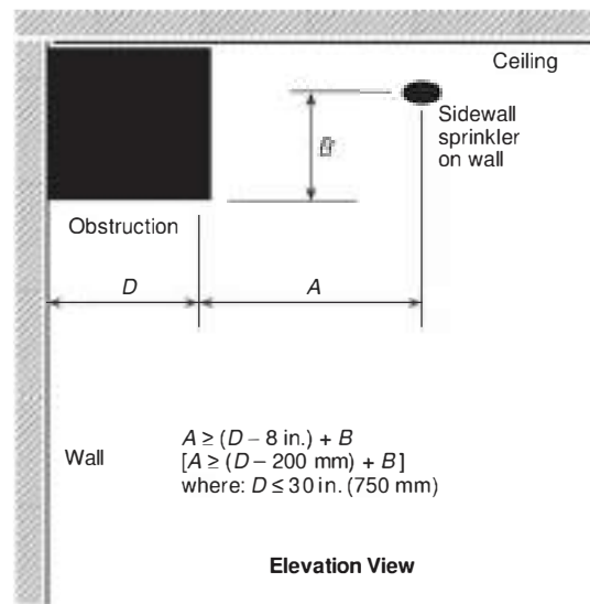
FIGURE 12.1.11.1.4(b) Obstruction Against Wall (Residential Sidewall Spray Sprinklers).
