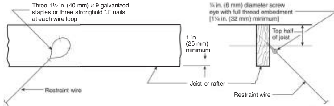
Detail A — Wood joist or rafter
