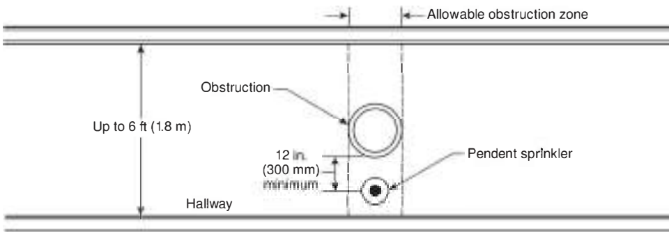
N FIGURE 12.1.10.1.2(d) Obstruction in Hallway.
