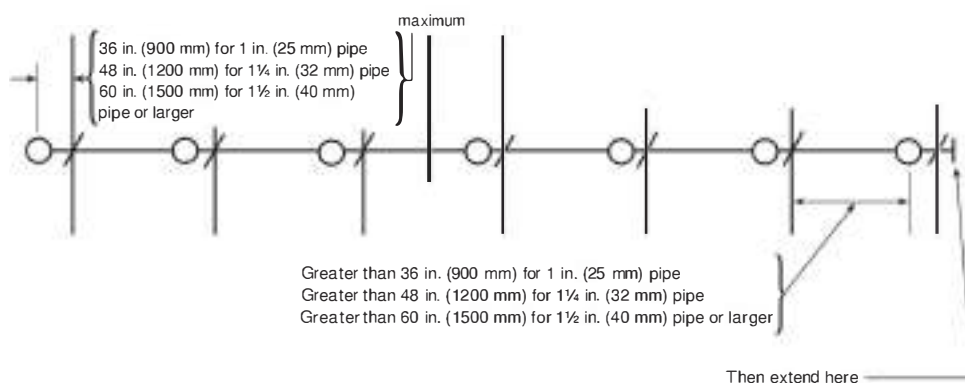
Δ FIGURE A.17.4.3.4 Distance from Sprinkler to Hanger.
