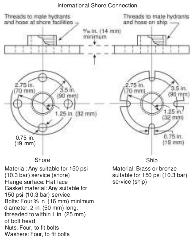
Δ FIGURE A.3.3.125.7 International Shore Fire Connection.
