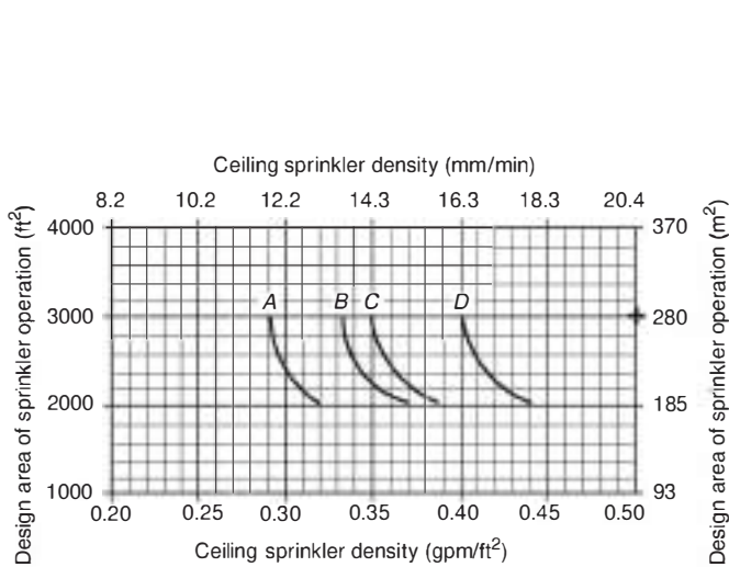
N FIGURE 25.8.2.2.1(c) CMDA Sprinkler System Design Curves — 20 ft (6.1 m) High Rack Storage — Exposed Nonencapsulated Class III Commodities — Conventional Pallets.
