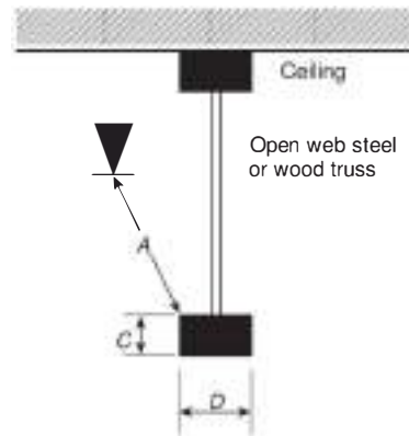
FIGURE 10.2.7.3.1.3(b) Minimum Distance from an Obstruction in the Horizontal Orientation (SSU/SSP).
