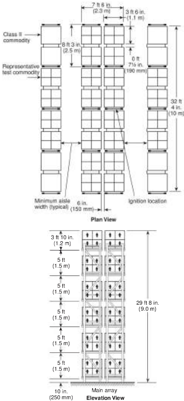
Δ FIGURE A.24.3 Typical Example of 30 ft (9.1 m) Double-Row Rack Storage Fire Test Arrangement.
