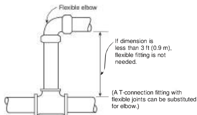
FIGURE A.18.2(b) Detail at Short Riser.
