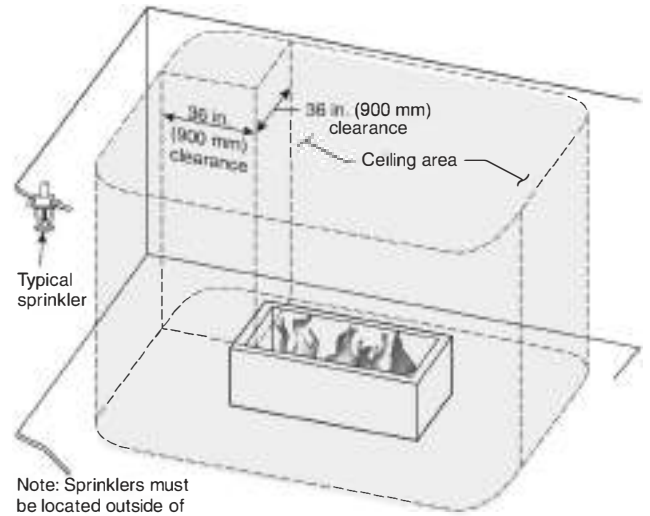
FIGURE A.9.4.2.5(c) Ordinary-Temperature Sprinkler over Open Fireplace.
