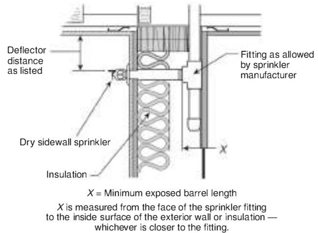
N FIGURE A.15.3.1(e) Dry Sidewall Sprinkler Through Wall.
