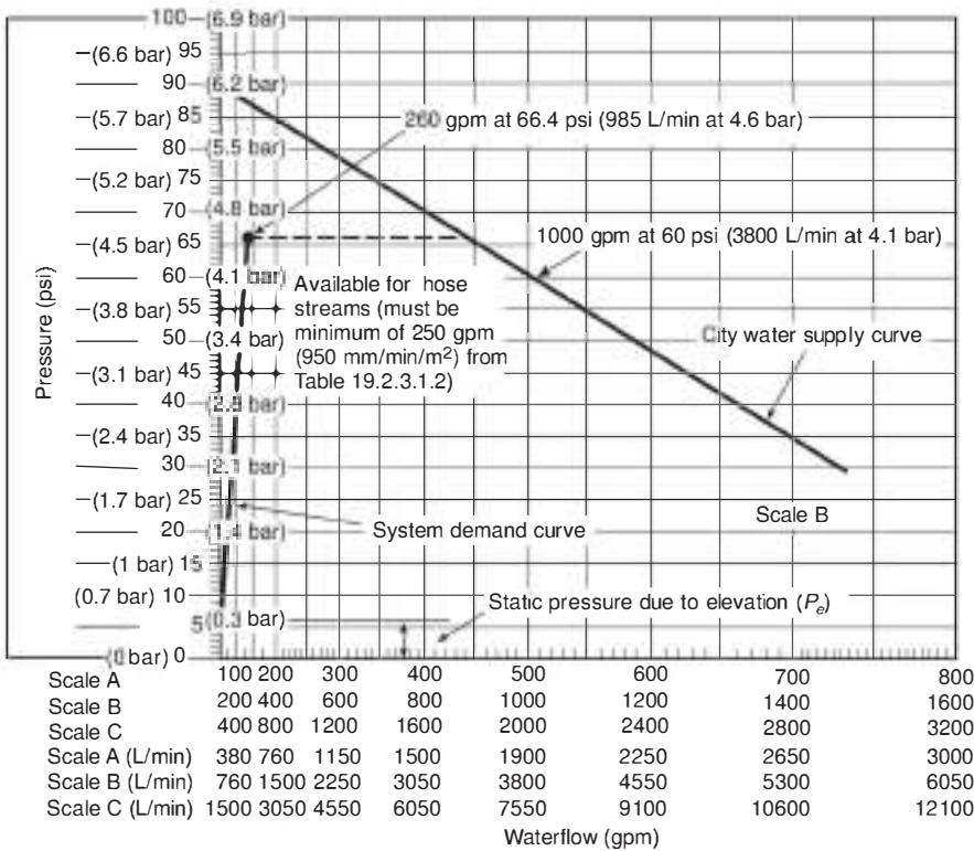
Δ FIGURE A.28.4.2(d) Hydraulic Graph.
