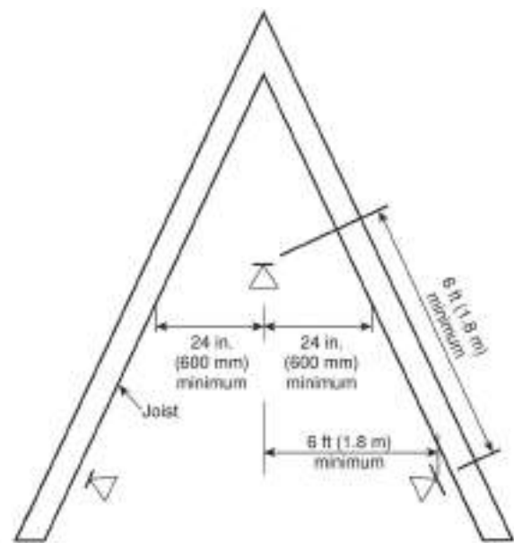
Δ FIGURE 10.2.6.1.3.3 Horizontal Clearance for Sprinkler at Peak of Pitched Roof.
