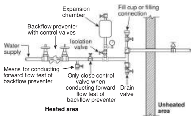
Δ FIGURE 8.6.3.3 Arrangement of Supply Piping with Backflow Device.
