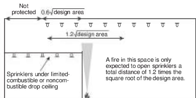
FIGURE A.9.3.14.3 Extension of Sprinkler System Above Drop Ceiling.
