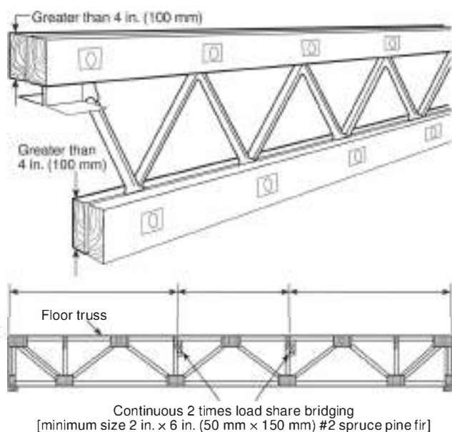
Δ FIGURE A.3.3.43.1(c) Wood Truss Construction.
