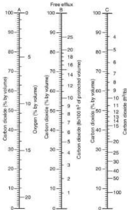
FIGURE D.1(b) Carbon Dioxide Requirements for Inert Atmospheres [based on a carbon dioxide expansion of 8.35 \text{ ft}^3/\text{lb} ( 0.52 \text{ m}^3/\text{kg} )].
