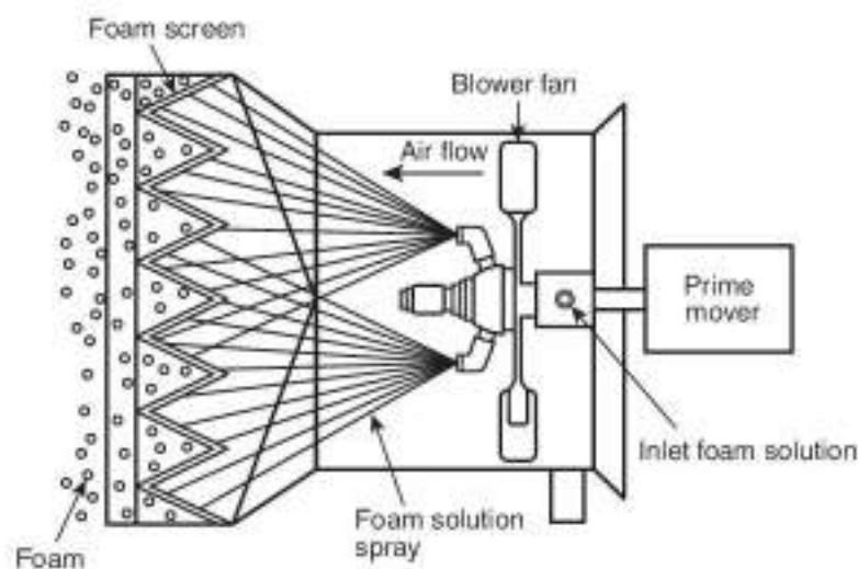
FIGURE A.7.7.4(c) Blower-Type Foam Generators.
