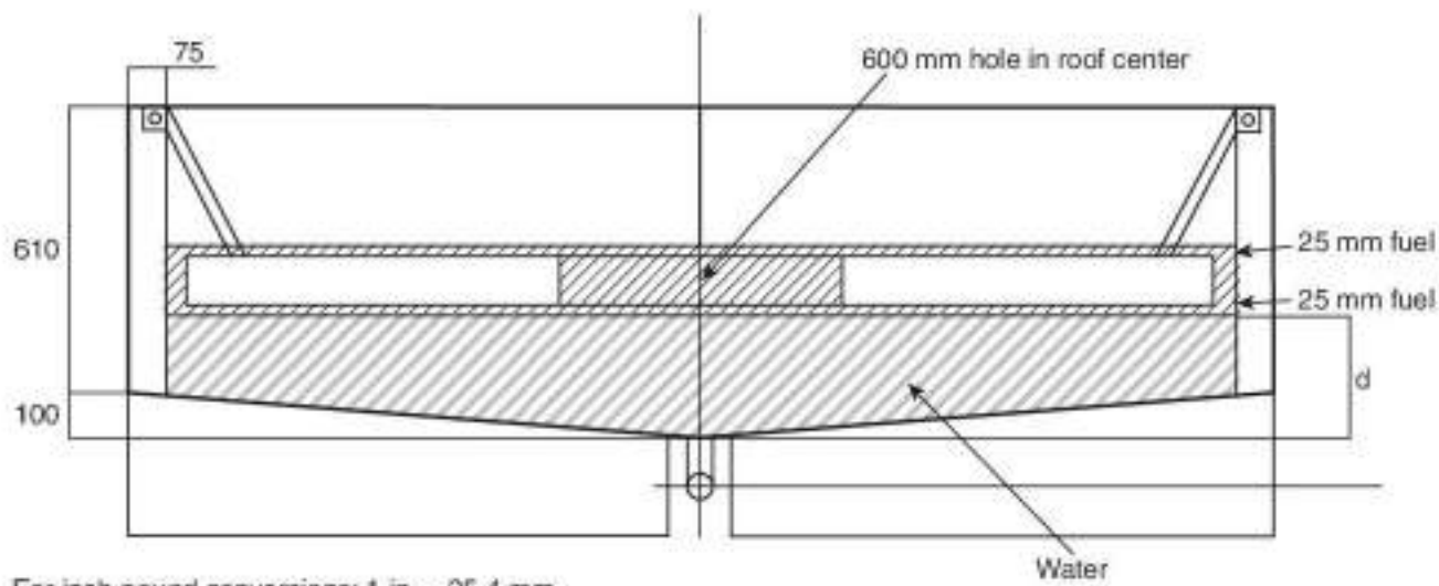
FIGURE I.1.2.1.1 General Layout of Roof Test.
