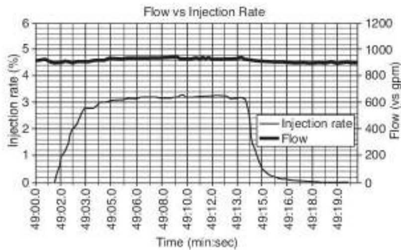
FIGURE D.5.2.2(a) Plot of Real-Time Test Data Gathered from Surrogate Liquid Injection Rate Test.
